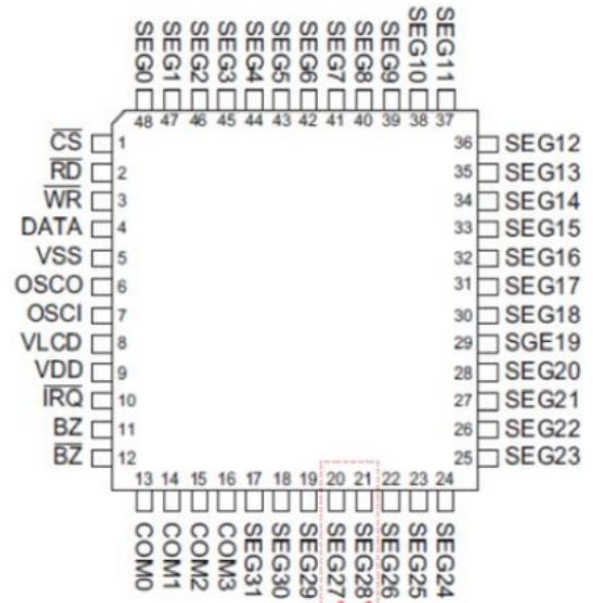
LQFP-48
