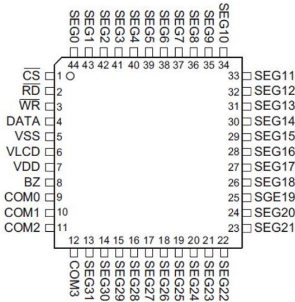
LQFP-44
