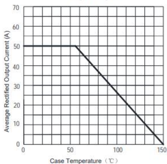
FIG1:Io-Tc Curve
