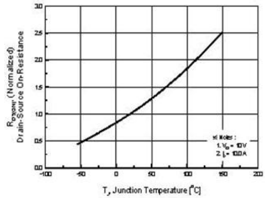
Figure 8. On-Resistance Variation
