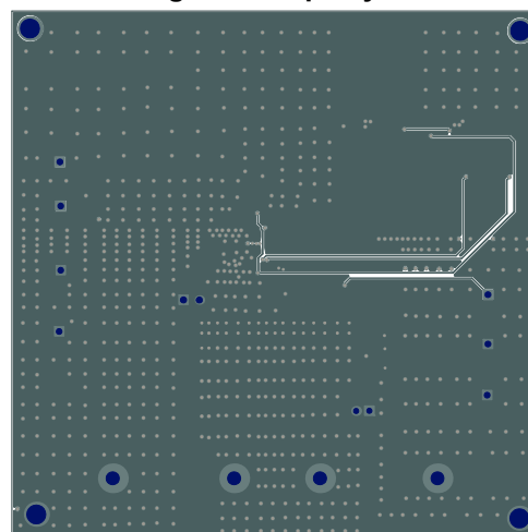
Figure 4: Middle2 Layer
