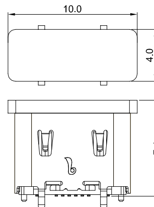
WITH COVER SCHEMATIC
