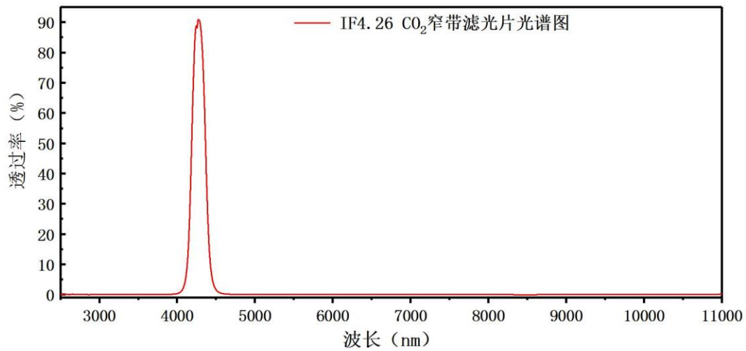
Transmittance of 4.26 \mu m Filter
