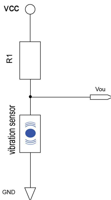
Figure 3: Basic circuit
