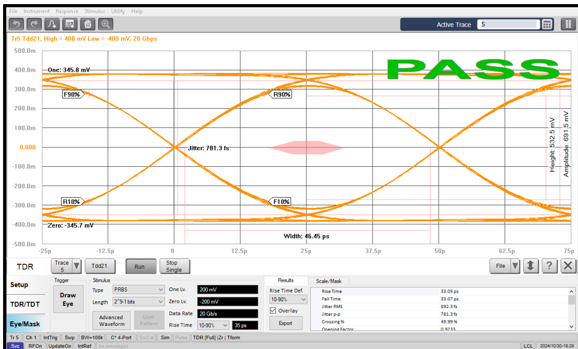
20 Gbps USB4 Eye Diagram
