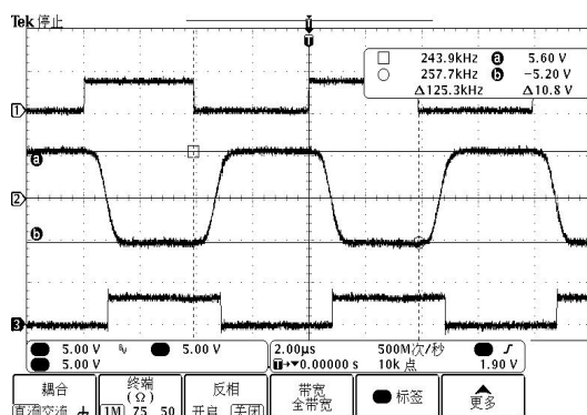
图 1. WS13232E TIN to TOut (no load) at 250kbps waveform
