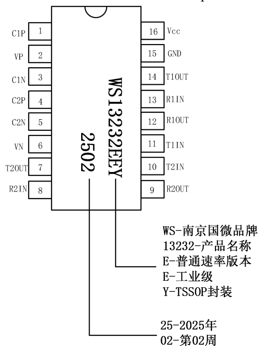
WS13232E 引脚图—16-pin SOP (Top View)
