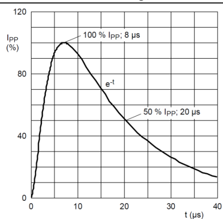
8/20 μs pulse waveform according to IEC 61000-4-5
