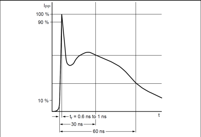
ESD pulse waveform according to IEC 61000-4-2
