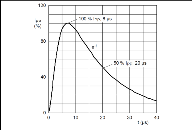
8/20 \mu s pulse waveform according to IEC 61000-4-5
