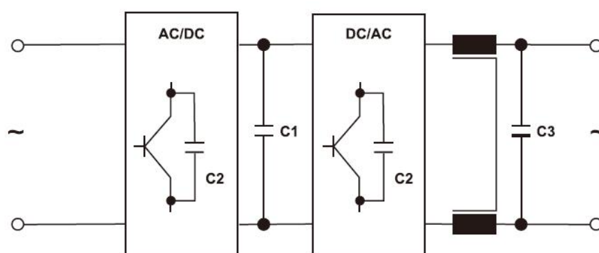
AC-Filter Capacitor (C3)
