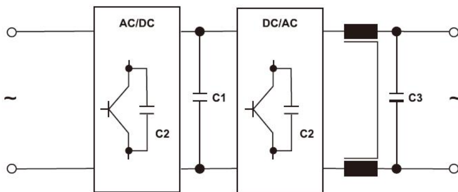
AC-Filter Capacitor (C3)
