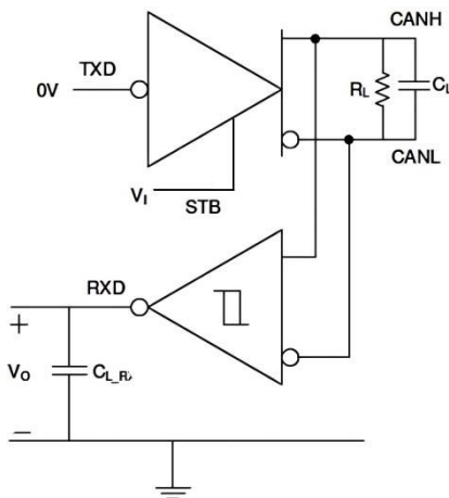
tMODE Test Circuit and Measurement
