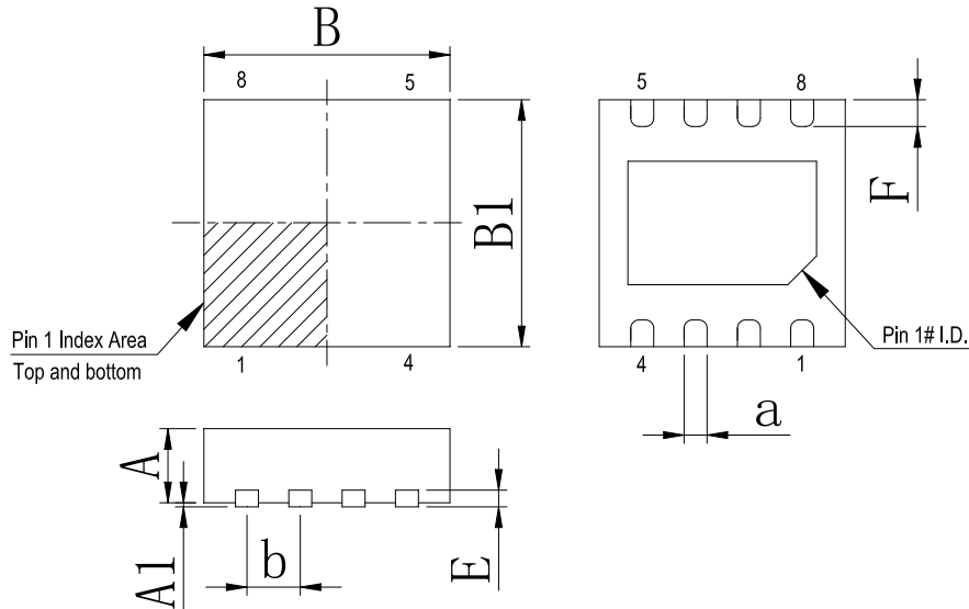
Dimensions In Millimeters(DFN-8 3*3)
