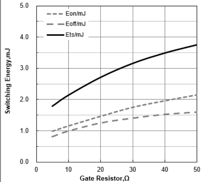
Figure 10. Typical Switching Energy vs Gate Resistor ( T_J=25^{\circ}\text{C} , V_{CE}=400\text{V} , V_{GE}=15/0\text{V} , I_C=50\text{A} )
