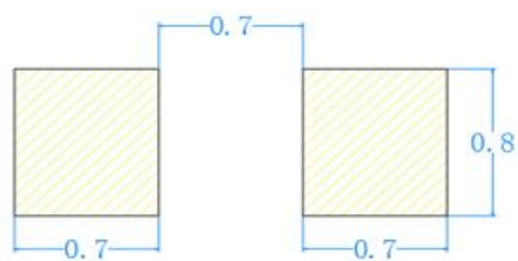
建议焊盘尺寸 Recommended Soldering Pattern
