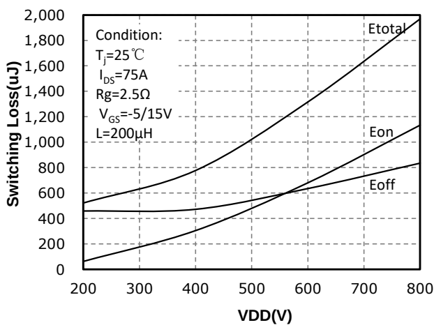
Fig 22: V_{DD}(\text{V}) vs. Switching Loss(uJ)
