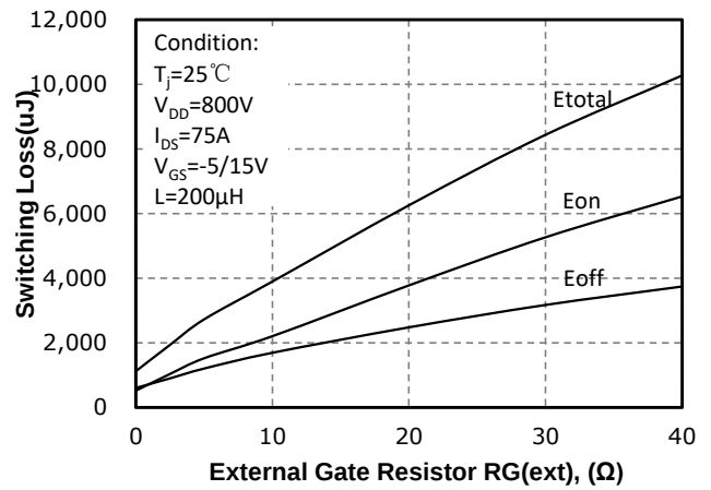
Fig 19: R_g(\Omega) vs. Switching Loss(uJ)
