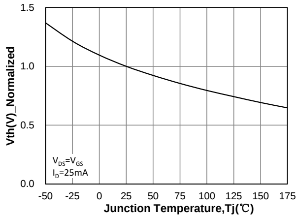
Fig 9: V_{th}(V) Vs T_j Characteristics
