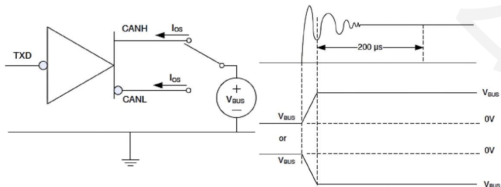
Driver Short Circuit Current Test and Measurement
