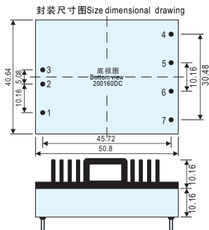
封装尺寸图Size dimensional drawing
