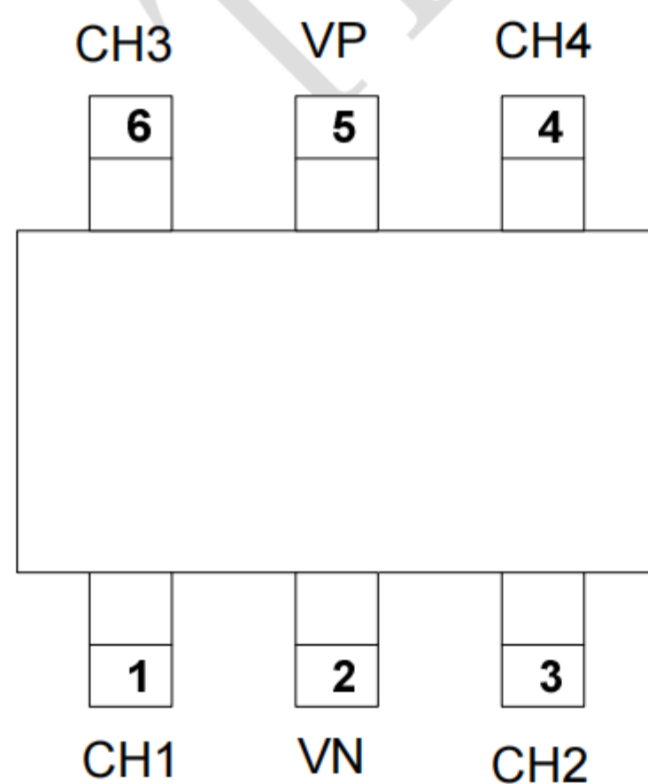
Circuit and Pin Schematic
