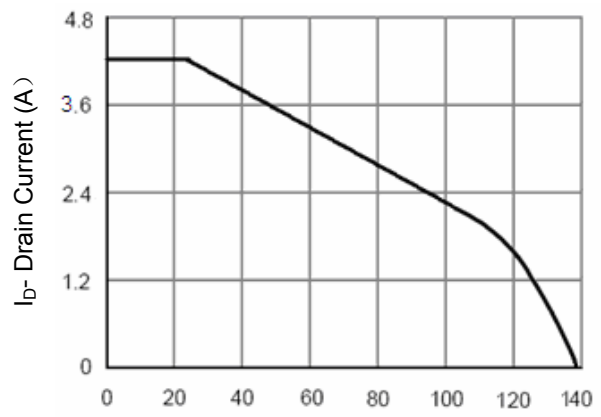
Figure 4 Drain Current
