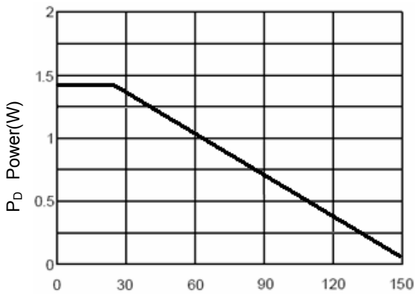
Figure 3 Power Dissipation
