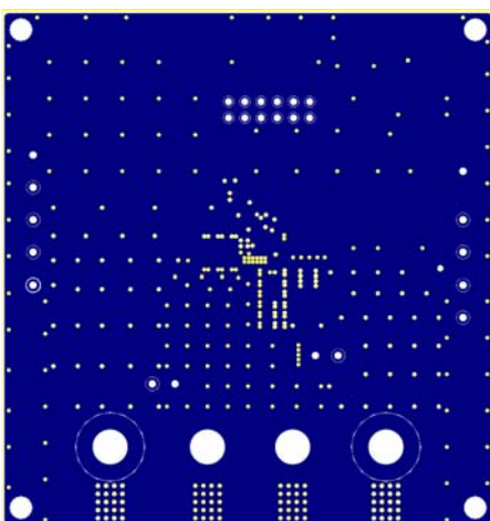
Figure 3—Inner Layer 1
