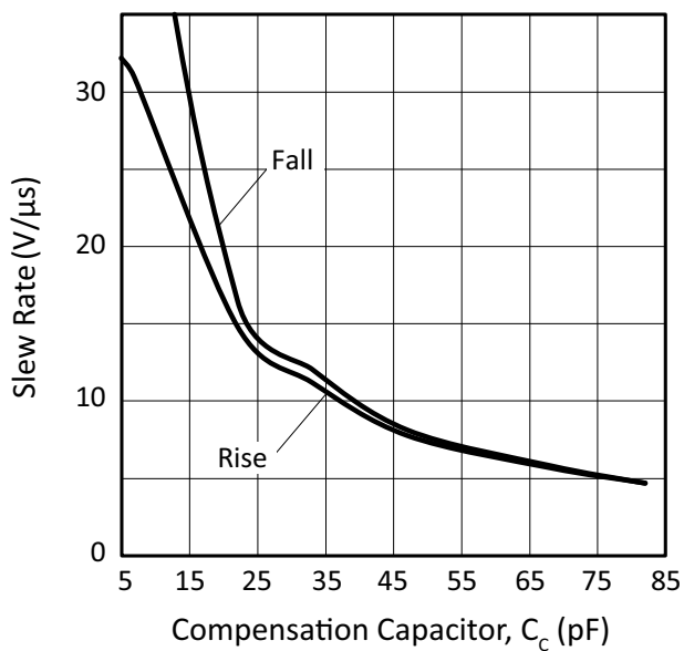
Figure 11: Slew Rate
