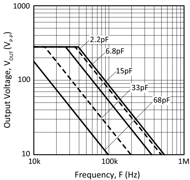
Figure 11: Slew Rate
