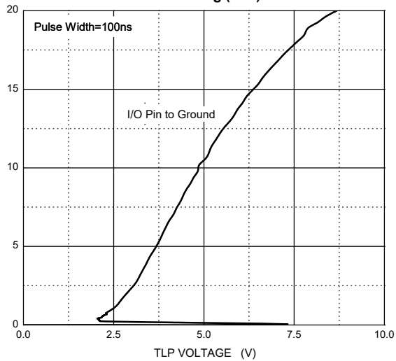
Transmission Line Pulsing (TLP) Measurement
