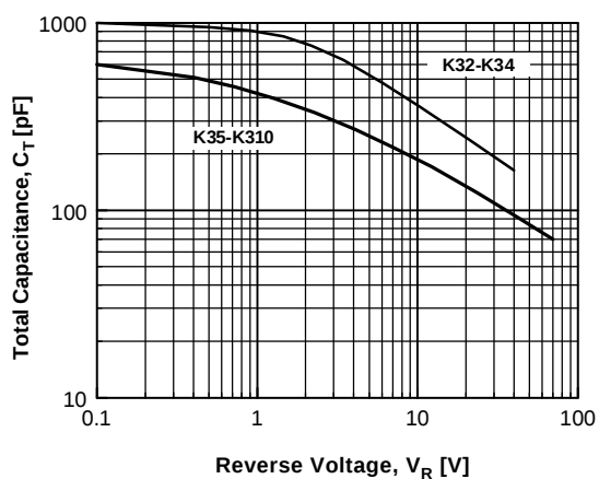
Figure 5. Total Capacitance
