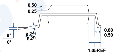
LEFT-SIDE VIEW
