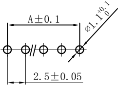
PCB LAYOUT
