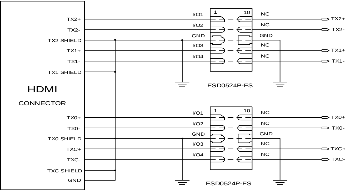
Typical HDMI Interface Application
