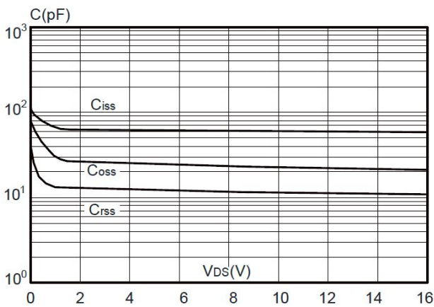
Figure 5: Capacitance Characteristics
