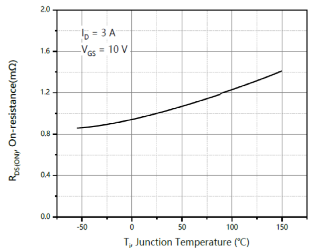
Figure4. Normalized On-Resistance
