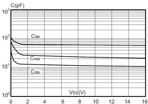
Figure 5: Capacitance Characteristics
