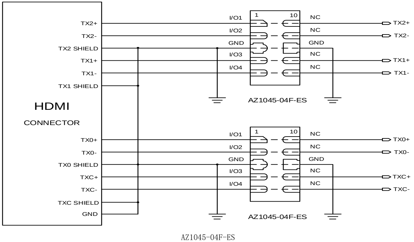
Typical HDMI Interface Application
