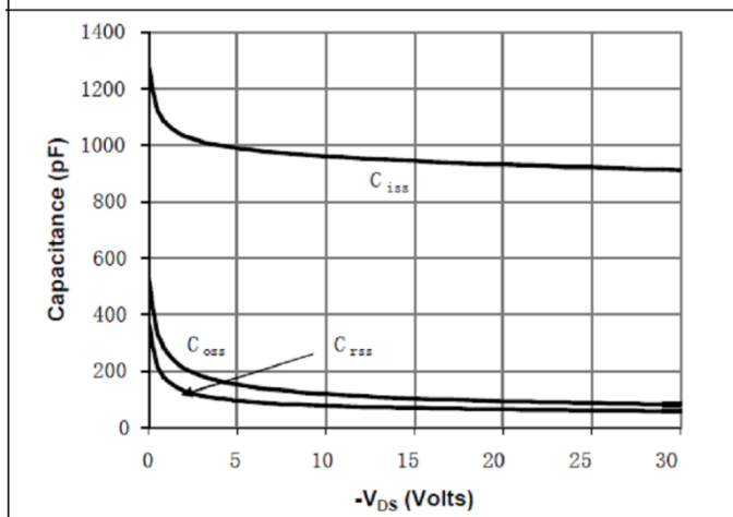
Figure 7. Capacitance Characteristics
