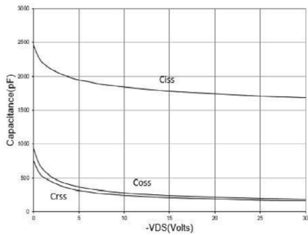
Figure 7. Capacitance Characteristics
