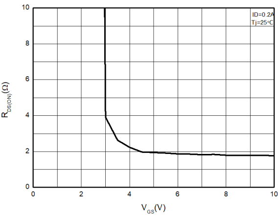
Figure 7: on-Resistance vs. Gate to Source
