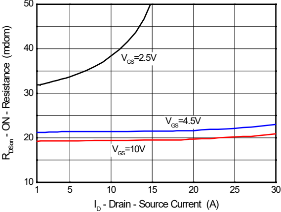
Figure 6. Rdson-Drain Current
