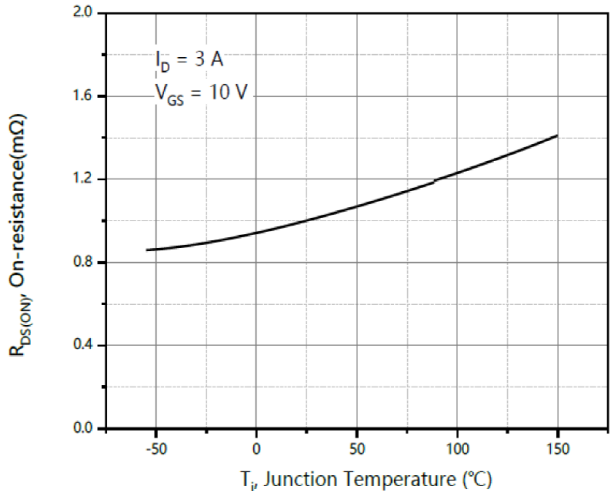
Figure6. Normalized On-Resistance
