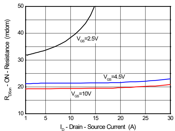
Figure 6. R_DS(on)-Drain Current
