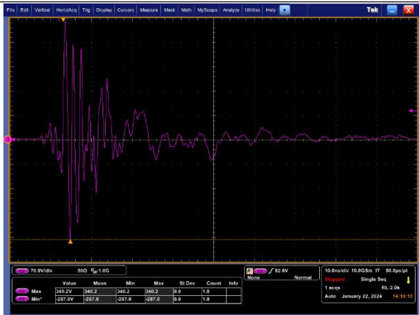
IEC6100-4-2 -15kV IO-IO
