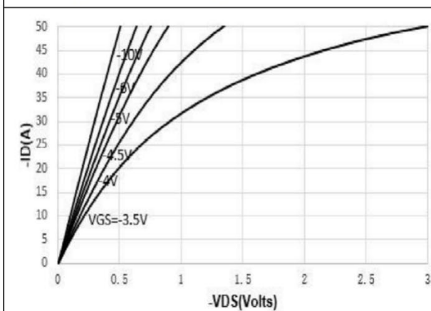
Figure 1. On-Regin Characteristics
