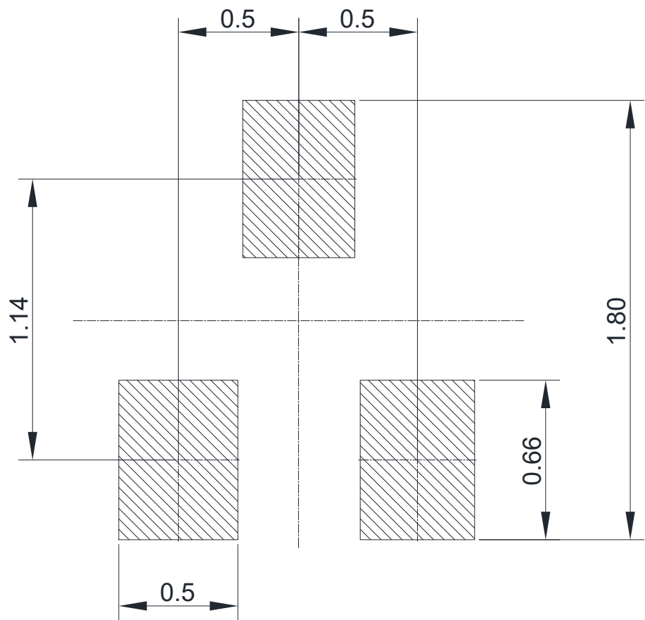
DIMENSIONS: MILLIMETERS
