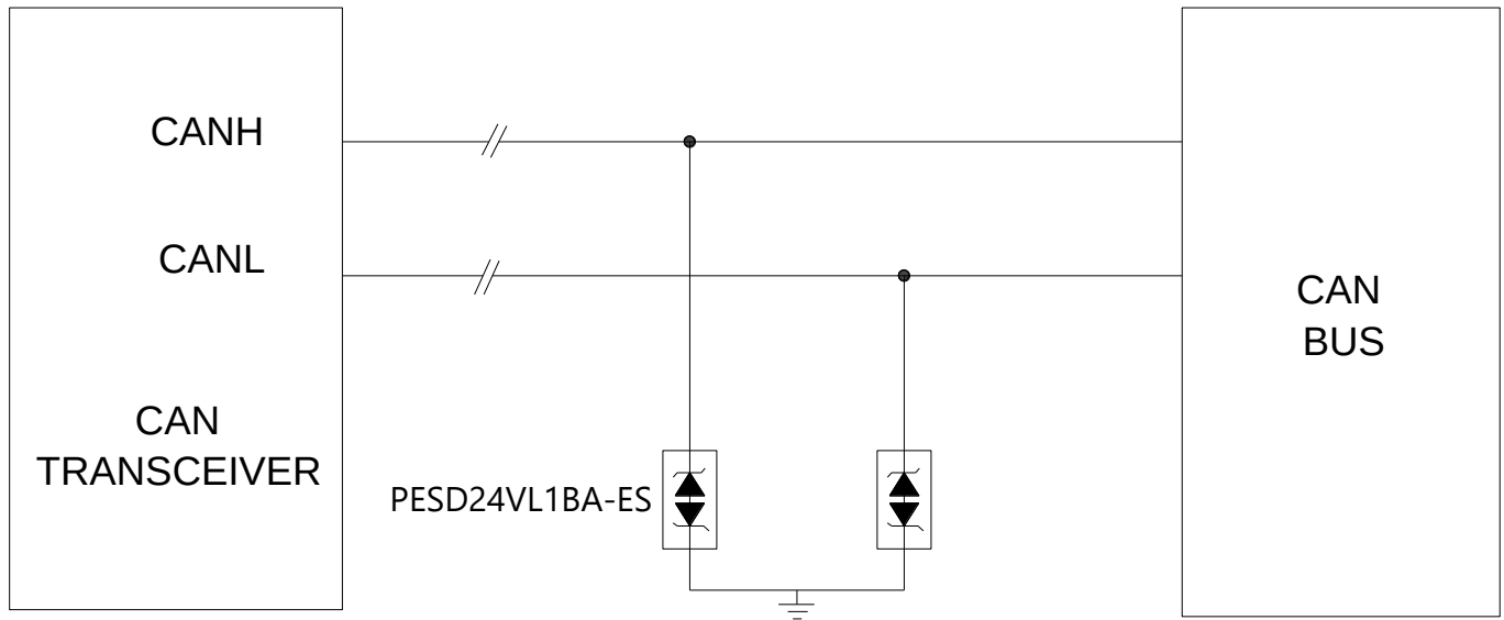
Typical Interface Application of CAN Bus Protection
