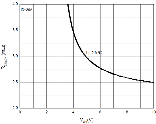
Figure4: on-Resistance vs. Gate to Source
