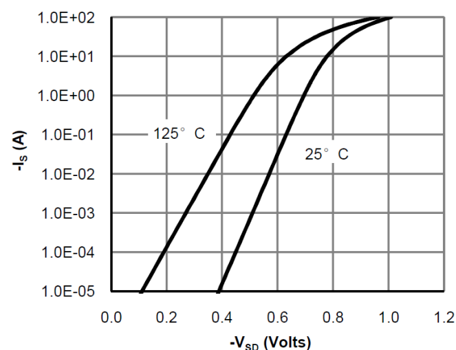
Figure 6: Body-Diode Characteristics
