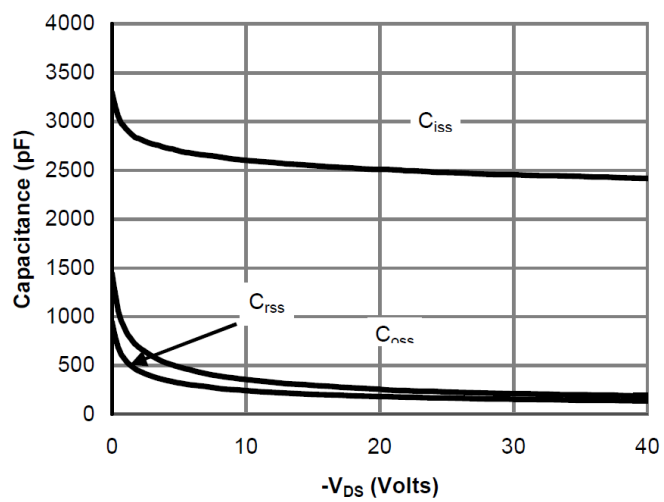
Figure 7: Capacitance Characteristics
