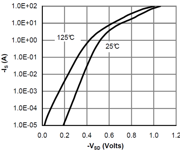
Figure 6: Body-Diode Characteristics
