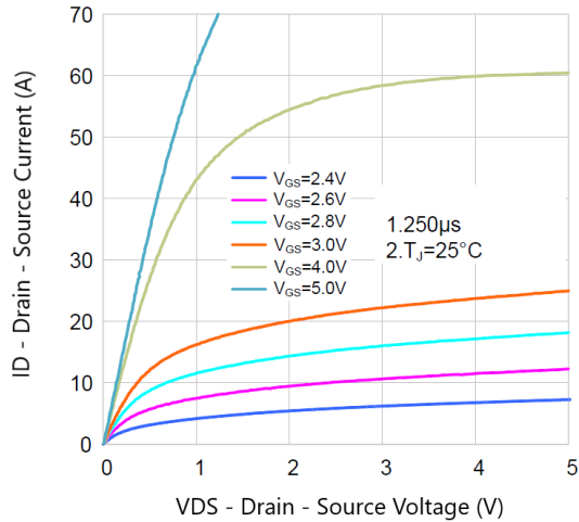
Figure 1. Typ. Output
