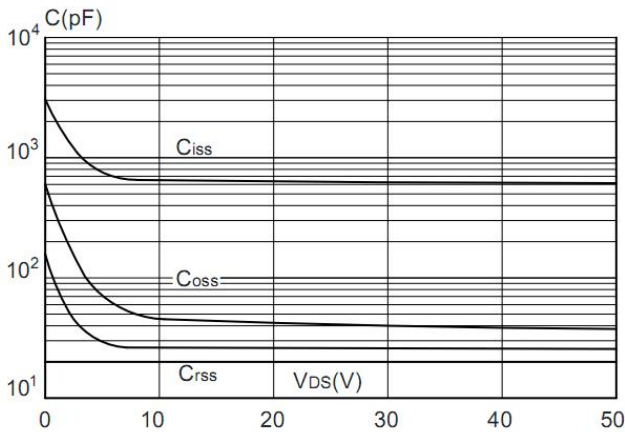
Figure 5: Capacitance Characteristics
