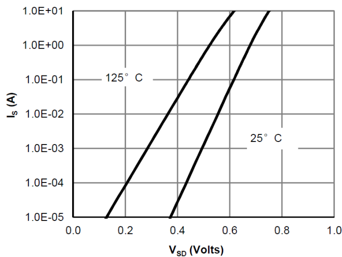
Figure 6: Body-Diode Characteristics
